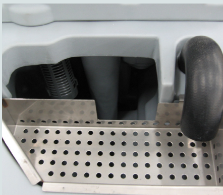
Recovery tank inlet system (180 degree recovery diverter + debris tray), for a quicker a more efficient cleaning
